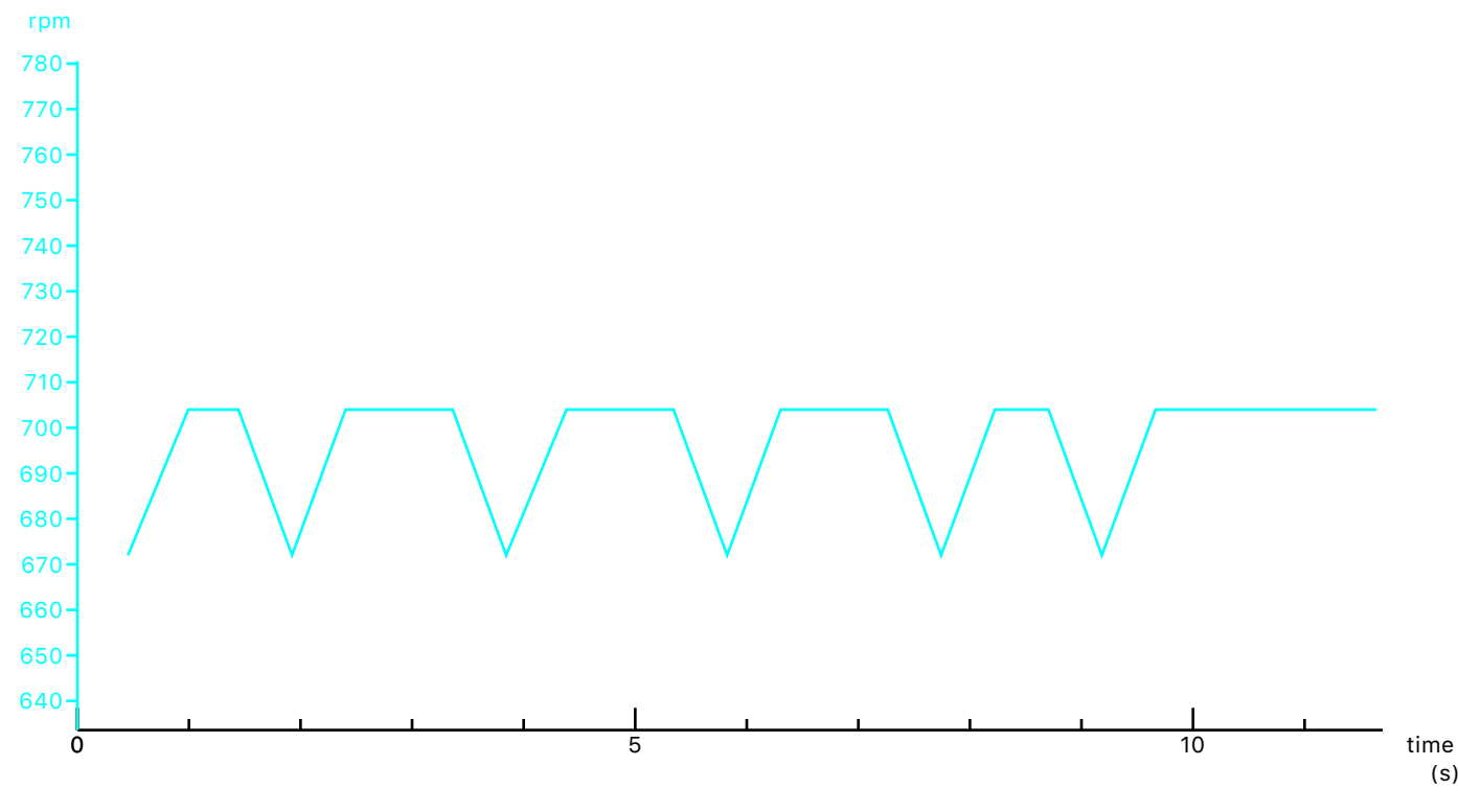
Engine speed
